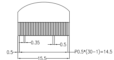
DETAIL B SCALE 4:1
